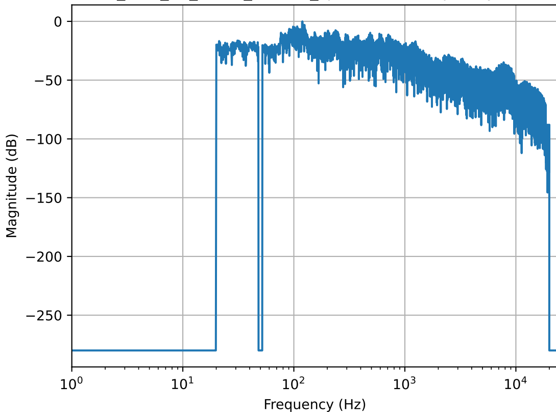
Daniel_5cm_03_linear_filtered_spectrum - Frequency Domain
