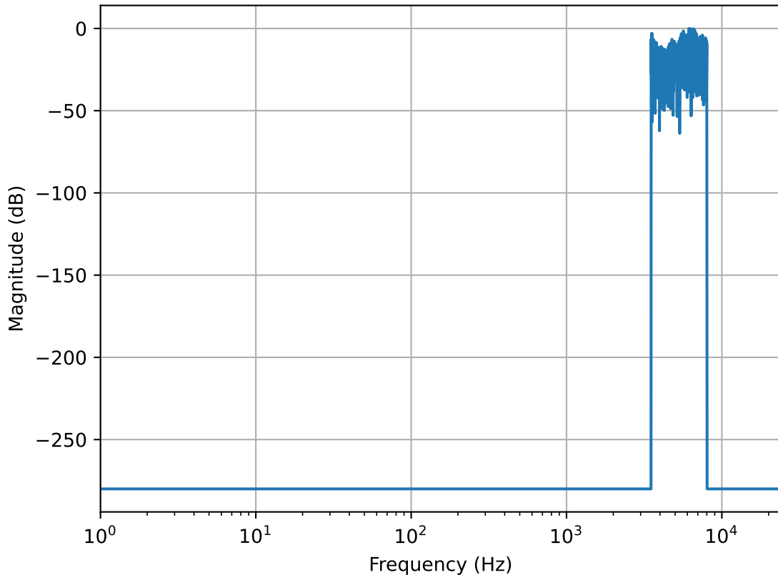
Daniel_5cm_06_upper_band_after_tanh - Frequency Domain
