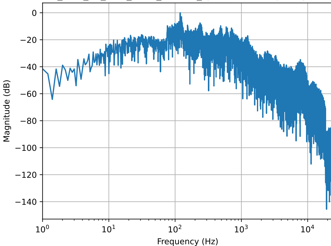
Daniel_5cm_08_final_aural_excited_spectrum - Frequency Domain
