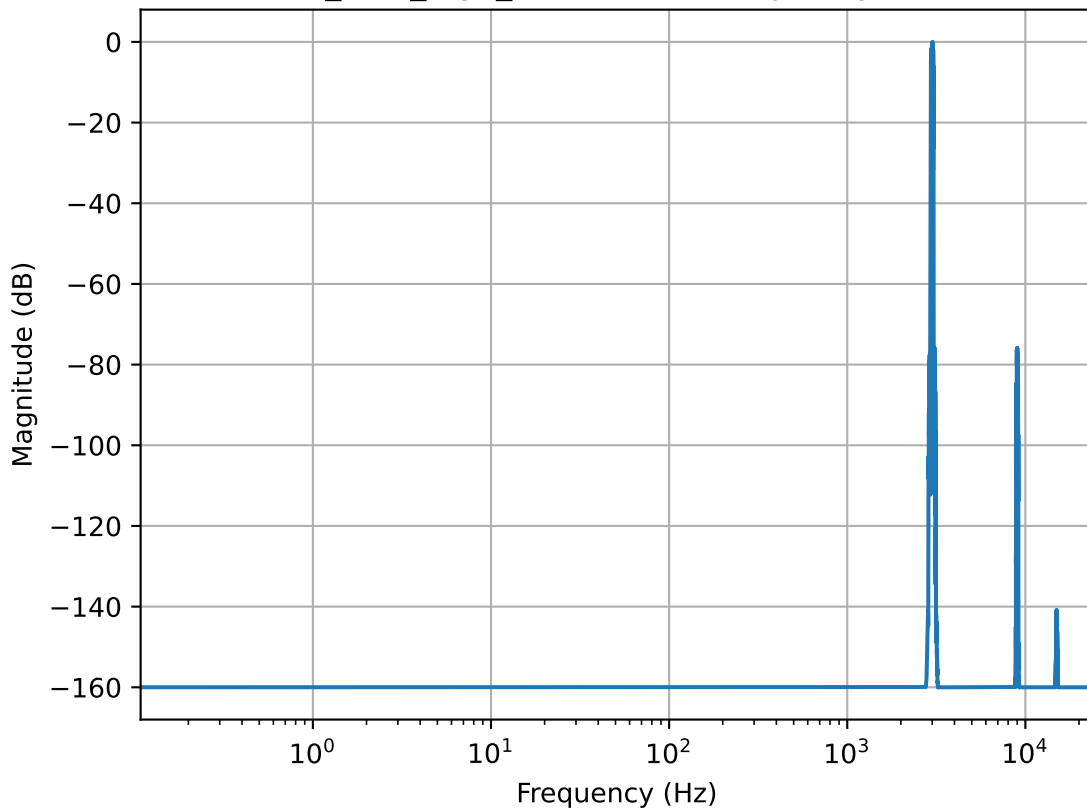
Daniel_5cm_high_harmonics - Frequency Domain
