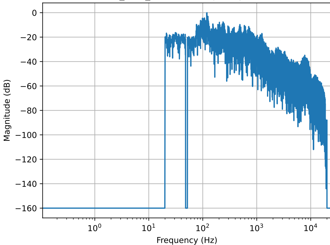
Daniel_5cm_filtered - Frequency Domain
