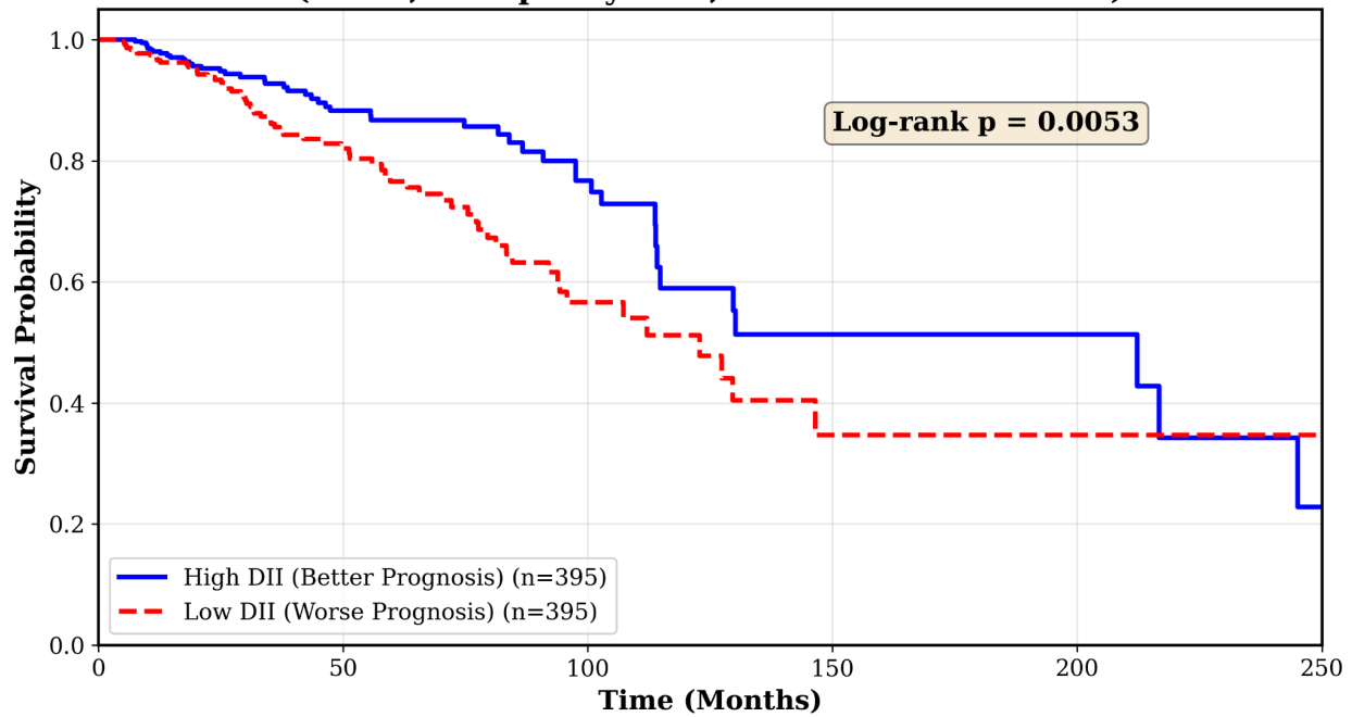
FIG. 2: Survival Stratification by DII Triplet (BRCA, Aneuploidy 5-25, CXCL13+ARG1+CD8A)
