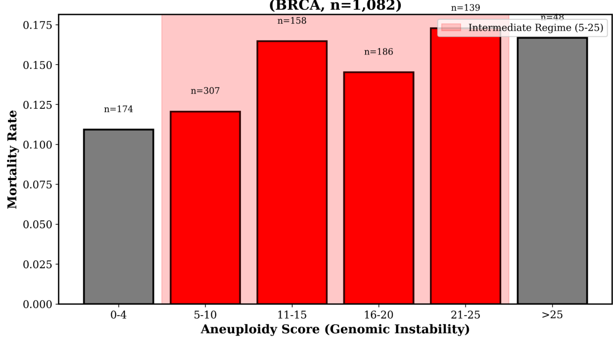
FIG. 1: The Intermediate Instability "Trap" (BRCA, n=1,082)
