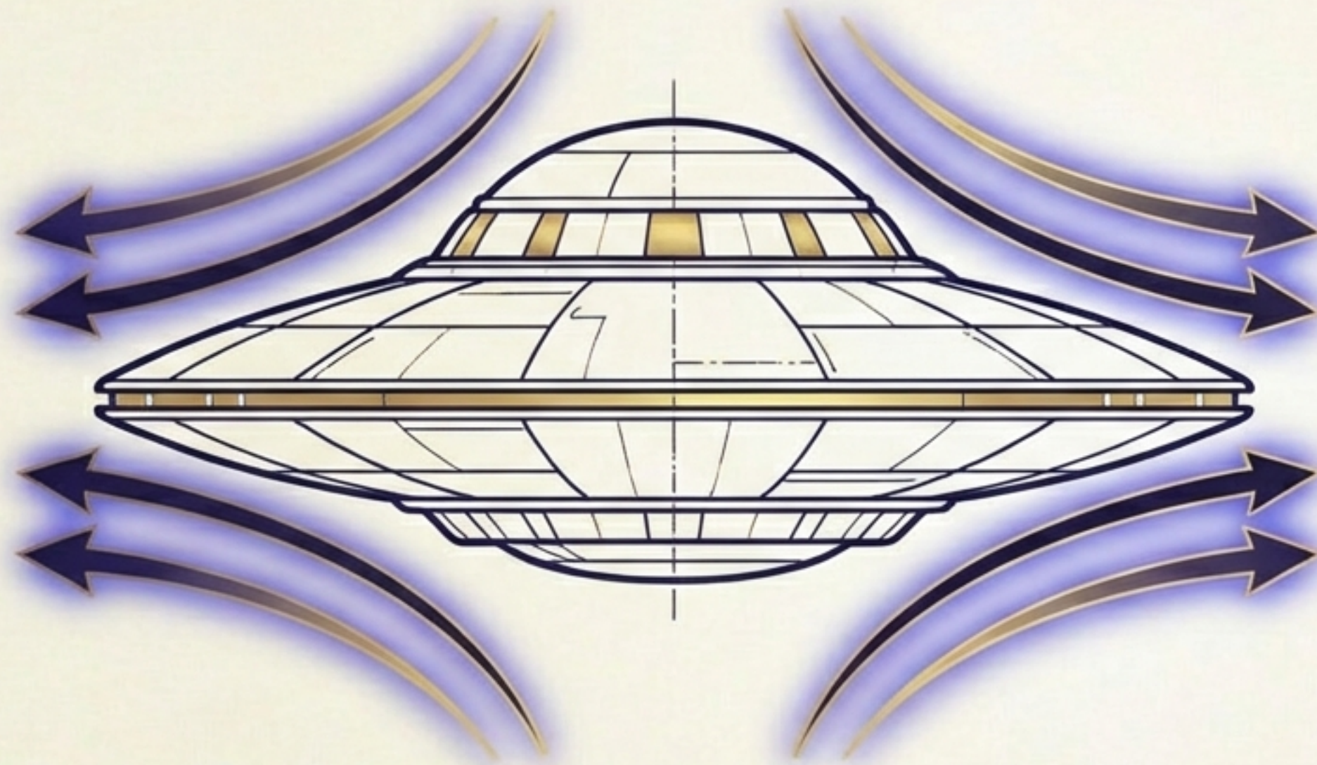
Meissner Field / Mass Cancellation
