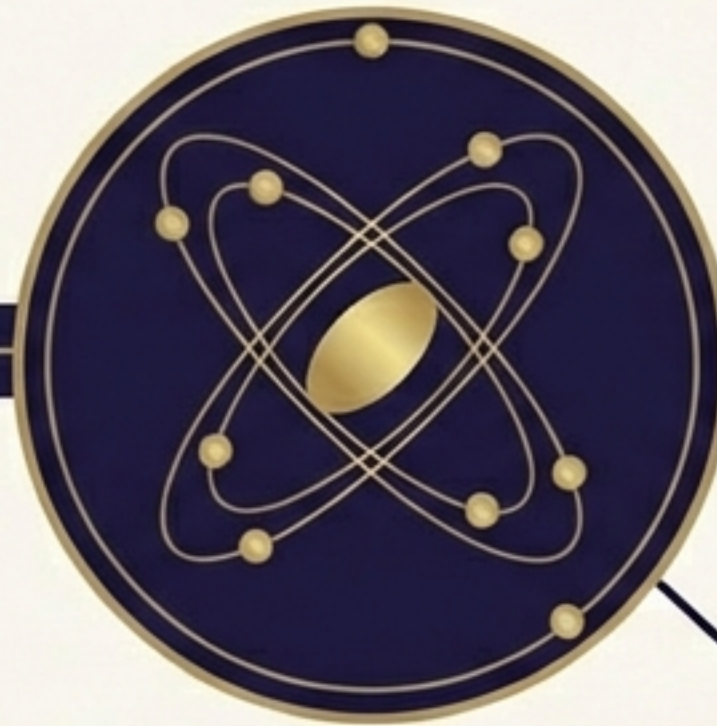
High-Spin State (ORMEs)
