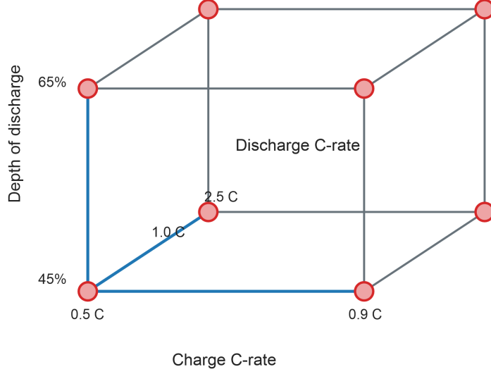
Figure 2: Three-factor design space of the LFP DoE Cycle Ageing Dataset. The cube axes show the low and high levels of charge C-rate, discharge C-rate, and depth of discharge. The eight marked corners are the operating-point combinations across which the fifteen test cells are distributed.
