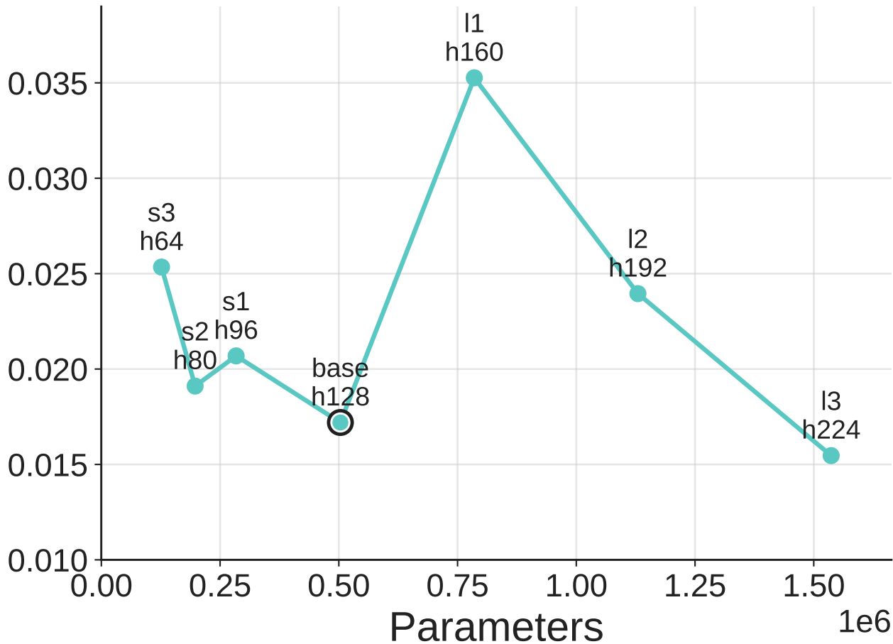
Cell-macro MAE
