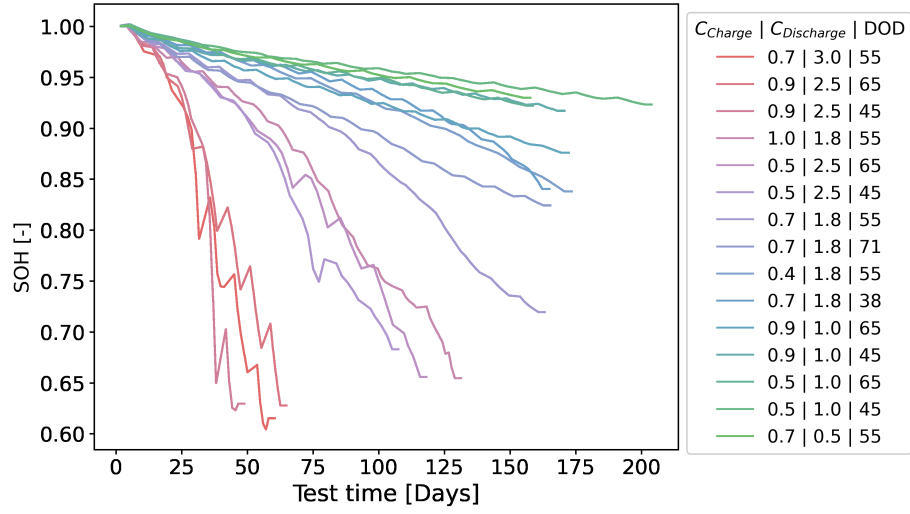
Figure A.25: Measured SOH trajectories across the complete LFP aging campaign. The campaign is divided into a six-cell training set, a three-cell validation set, and a six-cell independent holdout test set. The legend reports the applied charge C-rate, discharge C-rate, and depth of discharge for each trajectory. The plotted SOH values originate from repeated capacity checkups and are interpolated between checkup anchors. The exact cell-to-set assignment and measured coverage are reported in Table A.4.
