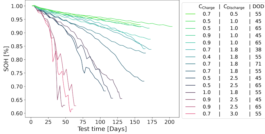
Figure 1: Capacity-based SOH reference trajectories of the 15 LFP cells over the aging campaign. Colors denote the investigated combinations of charge rate, discharge rate, and depth of discharge. The trajectory spread provides the common data basis for training and comparing the four neural architectures.
