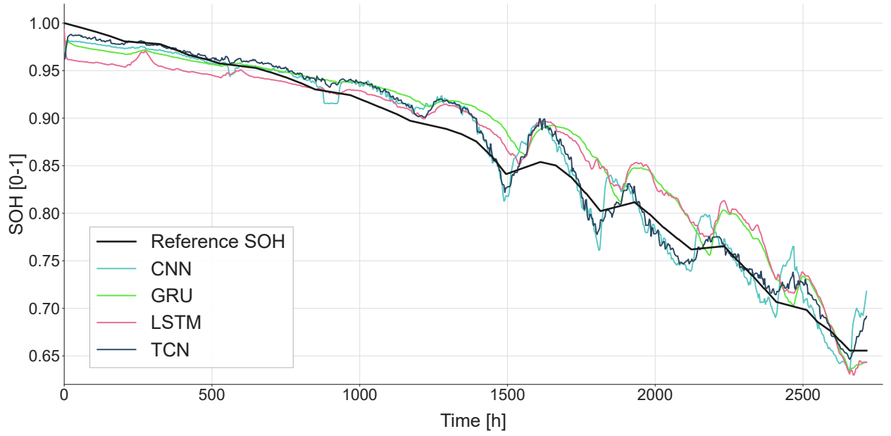
Figure 4: SOH trajectories of the selected uncompressed FP32 baseline models for one held-out test cell over 2716 hourly samples under continuous causal inference. The black line denotes the reference SOH, and the colored lines denote the predictions of the four architecture families. For legibility, the displayed prediction traces use a centered seven-hour median and every third plotting point. Smoothing and point reduction are applied only to this illustrative trajectory. The cell-macro errors in Figure 3(a) are calculated from unsmoothed model outputs across all three test cells.
