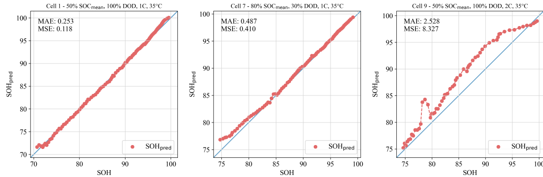
Figure 4.6: Scatter comparison between predicted and measured SOH values for the three representative test cells. Cells 7 and 1 remain close to the identity line and therefore exhibit low prediction errors. For Cell 9, the model follows parts of the qualitative SOH development, but the larger distances from the identity line show that the absolute SOH values are reproduced less accurately. The atypical trajectory alone does not cause the error. MAE and MSE quantify the residual deviations between prediction and reference. Error values are shown on the 0 to 100% SOH scale, with MAE in percentage points and MSE in squared percentage points.
