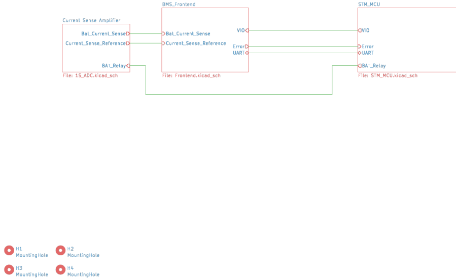
Figure 3.6: Reduced system-level block view of the Custom BMS Platform showing the interaction between current sensing, BMS front-end, and microcontroller domain.
