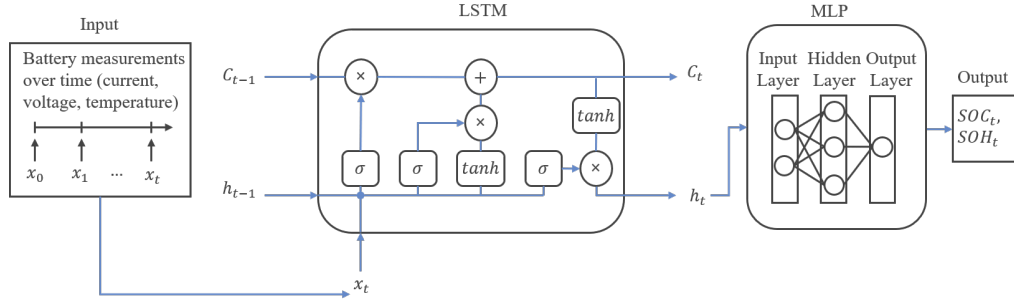
Abbildung 7.1: Stateful LSTM+MLP estimator structure used for both SOC and SOH estimation. Preprocessed feature streams are processed step by step by a single-layer LSTM whose hidden and cell states are propagated across time; a lightweight MLP head then maps the hidden representation to either SOC or SOH. The SOC instance uses hidden size 64 with an MLP width of 64 and a sigmoid output, the SOH instance hidden size 128 with an MLP width of 128 and a linear output. This structure is the basis for the later pruning, quantization, and MCU export steps.
