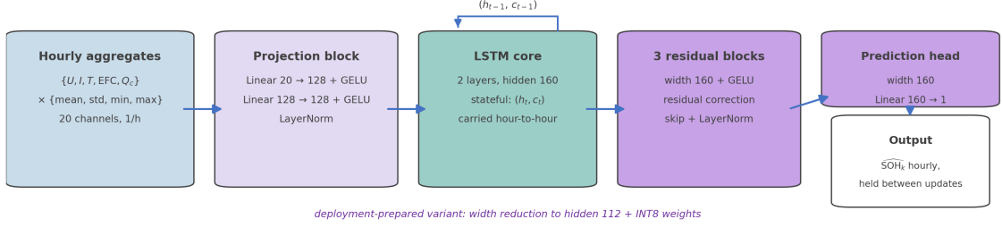
Figure 6.3: Block-level architectures of the data-driven estimator components used in the benchmark. (a) The DD SOC estimator processes the eight online input channels with a single stateful GRU layer of hidden size 96, followed by an MLP head with one ReLU-activated hidden layer of size 96 and a sigmoid output. (b) The shared SOH estimator forms a 20-dimensional hourly feature vector by computing four statistics for each of the five causal base signals \{U, I, T, \text{EFC}, Q_c\} , projects this vector through a two-layer feature-projection block of width 128, processes the projected sequence with a two-layer stateful LSTM of hidden size 160, and maps the recurrent representation through three residual MLP blocks and a prediction head of width 160. The deployment-prepared variants used in the benchmark are described in Section 6.5.4.
