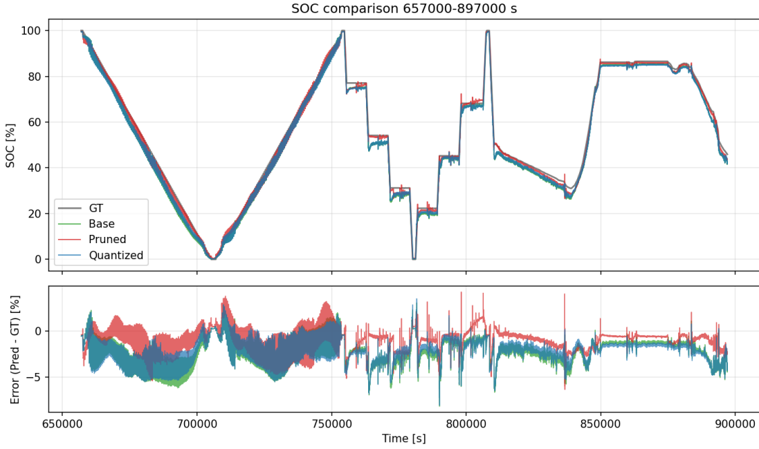
Figure 6.11: Detailed check-up-region analysis of embedded SOC streaming replay. The figure covers a representative diagnostic interval with long integration horizons and illustrates the stability of the stateful deployments during extended charge/discharge behaviour.
