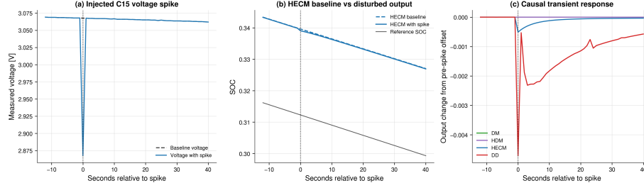
Figure 17: Causal single-cell voltage-spike response for C15 at mid-life. (a) Measured voltage with and without the injected spike, aligned to the true injection sample. (b) HECM output with its paired baseline and reference SOC. (c) Model-output change relative to the pre-spike paired offset.
