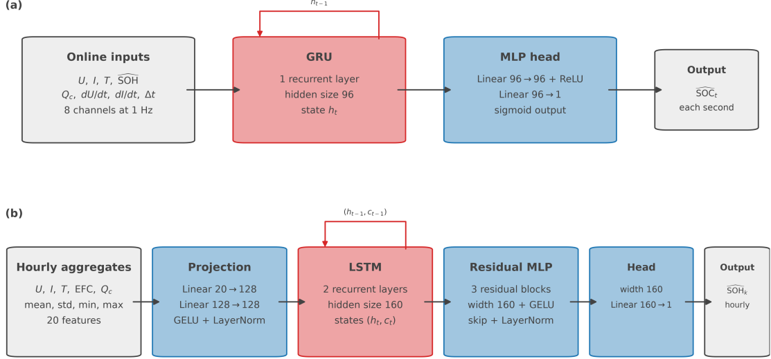
Figure 5.2: Block-level architectures of the data-driven estimator components used in the benchmark. (a) The DD SOC estimator processes the eight online input channels with a single stateful GRU layer of hidden size 96, followed by an MLP head with one ReLU-activated hidden layer of size 96 and a sigmoid output. (b) The shared SOH estimator forms a 20-dimensional hourly feature vector by computing four statistics for each of the five causal base signals \{U, I, T, \text{EFC}, Q_c\} , projects this vector through a two-layer feature-projection block of width 128, processes the projected sequence with a two-layer stateful LSTM of hidden size 160, and maps the recurrent representation through three residual MLP blocks and a prediction head of width 160. The deployment-prepared variants used in the benchmark are described in Section 5.2.4.
