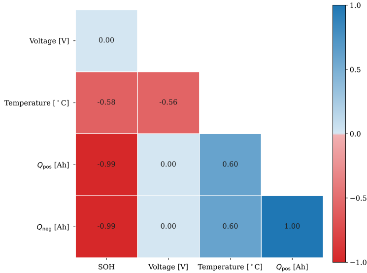
Figure 4.1: Correlation heatmap illustrating the linear relation between SOH and candidate input variables, including temperature and cumulative current Q in positive and negative direction. Correlation coefficients near +1 or -1 indicate strong linear dependence, whereas values near 0 indicate little or no direct linear relation.
