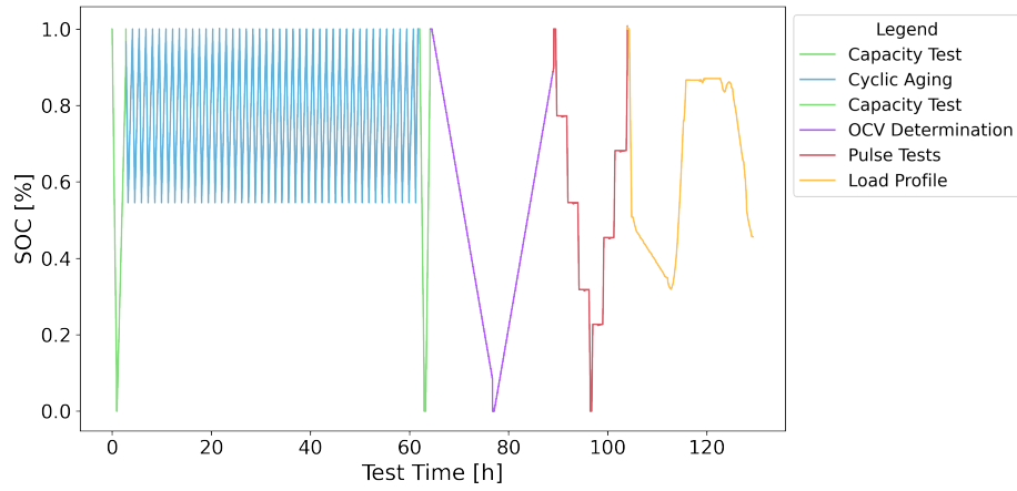
Figure 3.3: Representative SOC trajectory illustrating the experimental structure of the LFP campaign. The sequence combines cyclic ageing operation, diagnostic check-up blocks, and stationary-storage load-profile segments, capturing both laboratory reference phases and application-oriented dynamic behaviour.
