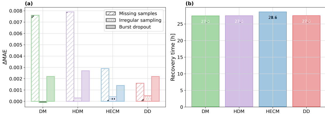
Figure 5.8: Continuity and timing disturbance summary. The figure compares the global \Delta\text{MAE} penalties for missing samples, irregular sampling, and burst dropout, and it complements these full-run penalties with the burst-dropout recovery times. This compact summary shows why missing samples, timing irregularity, and longer frozen-data gaps cannot be judged from one metric alone.
