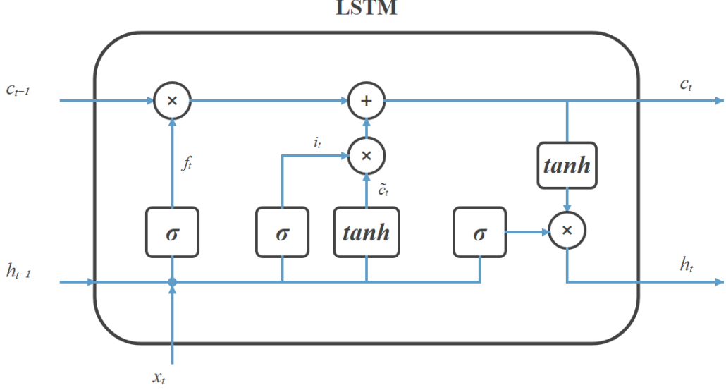
Figure 2.3: Detailed data flow through an LSTM cell corresponding to Equation (2.12). The forget gate controls the retained cell state, the input gate controls the candidate write operation, and the output gate controls the exposed hidden state. Blue paths indicate the directed state and gate signals, \odot denotes element-wise multiplication, and the addition node forms the updated cell state.
