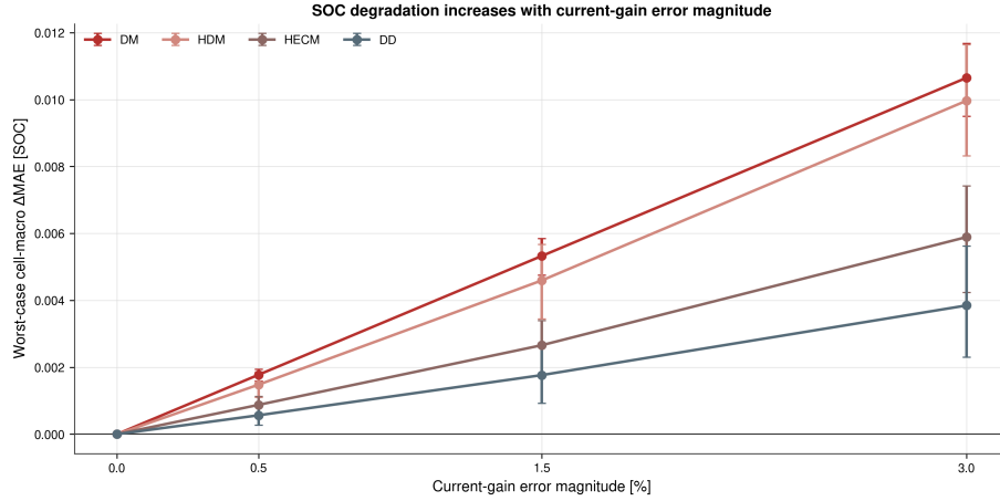
Figure 12: Worst-case sensitivity to current-gain error across the six independent holdout cells. For each gain-error magnitude and cell, the adverse direction from the matched \pm b pair is retained. Points show equal-weight cell-macro changes in MAE relative to each estimator's baseline; error bars show 95% bootstrap confidence intervals across cells.
