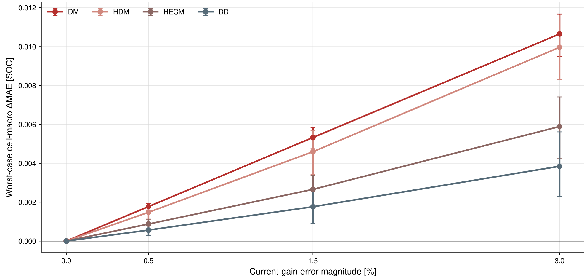
SOC degradation increases with current-gain error magnitude
