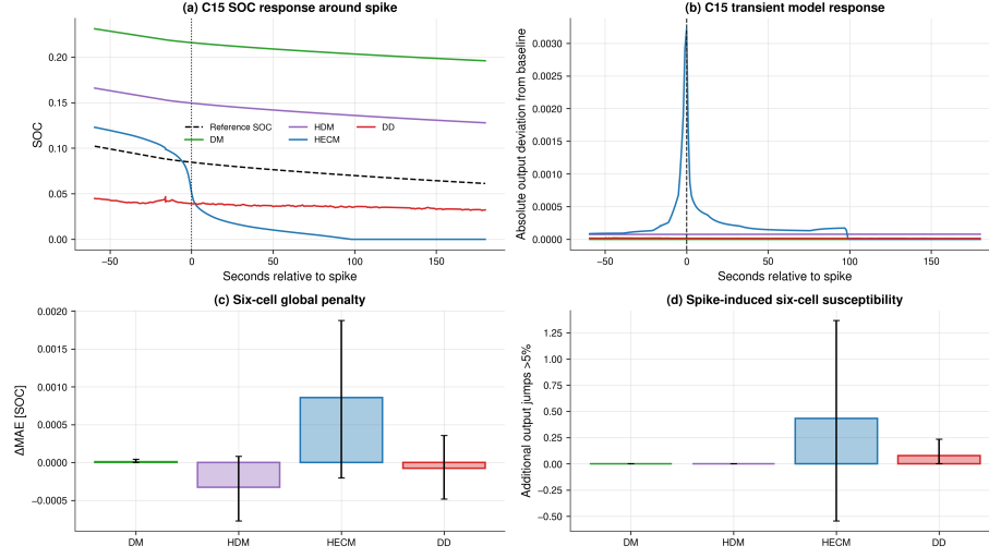
Figure 17: Voltage-spike sensitivity. (a) Representative C15 mid-life SOC response around a spike selected from the strongest HECM-response cell. (b) Absolute deviation of the disturbed output from its paired baseline output. (c) Six-cell global MAE penalty. (d) Additional output jumps above 5% relative to baseline; error bars show 95% bootstrap confidence intervals.
