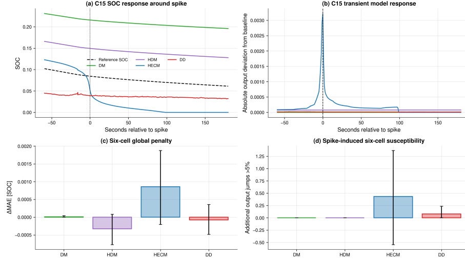
Figure 17: Voltage-spike sensitivity. (a) Representative C15 mid-life SOC response around a spike selected from the strongest HECM-response cell. (b) Absolute deviation of the disturbed output from its paired baseline output. (c) Six-cell global MAE penalty. (d) Additional output jumps above 5% relative to baseline; error bars show 95% bootstrap confidence intervals.
