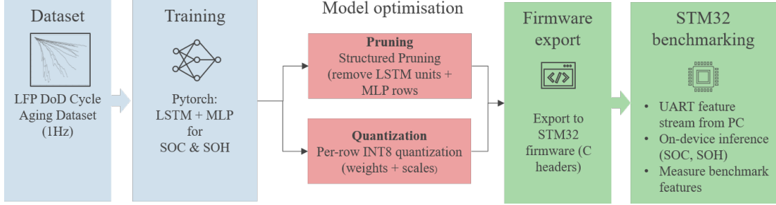
Figure 6.3: End-to-end deployment pipeline from the LFP ageing dataset and Py-Torch training to pruning, quantization, C-header export, and final STM32 benchmarking. The same trained SOC and SOH parameter sets form the basis of the floating-point, pruned, and quantized deployments, which keeps the later comparisons numerically consistent.
