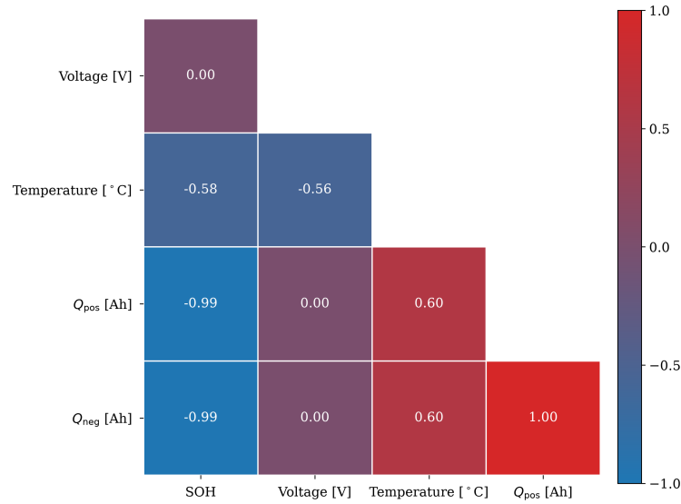
Figure 4.1: Correlation heatmap illustrating the linear relation between SOH and candidate input variables, including temperature and cumulative current Q in positive and negative direction. The continuous sRGB scale maps negative correlations to blue and positive correlations to red, with the direct blue-red mixture representing zero. The exact coefficient is printed in each cell.
