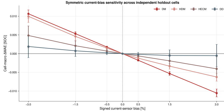
Figure 12: Symmetric current-offset sensitivity across the six independent holdout cells. Points show equal-weight cell-macro changes in MAE relative to each estimator's baseline; error bars show hierarchical 95% bootstrap confidence intervals. Negative offsets reinforce the positive baseline errors of DM and HDM, whereas positive offsets partially compensate them.
