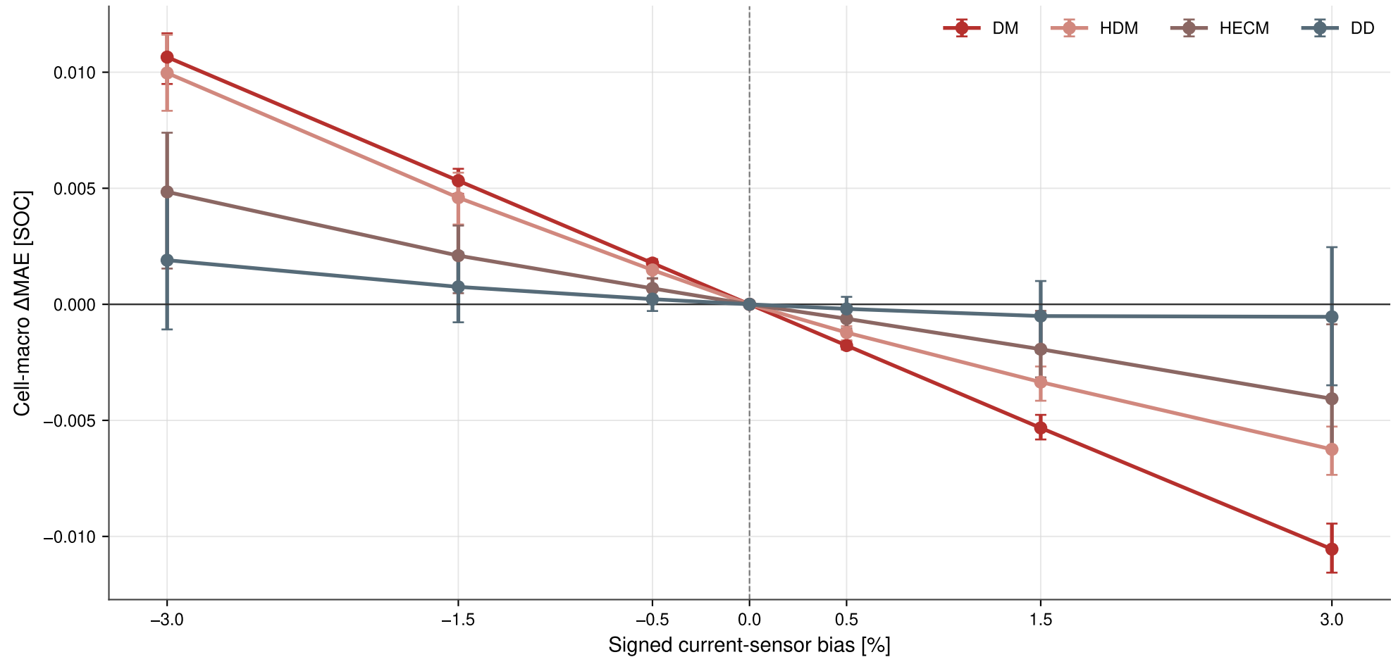
Symmetric current-bias sensitivity across independent holdout cells
