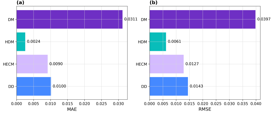
Figure 4: Baseline performance on the selected full-cell benchmark trajectory. The hybrid direct-measurement model provides the lowest clean-condition error, whereas the direct-measurement model shows the largest baseline deviation.
