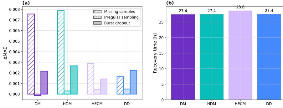
Figure 8: Signal-integrity performance summary. The left panel compares the global MAE penalties for missing samples, irregular sampling, and burst dropout, whereas the right panel summarizes the burst-dropout recovery time.
