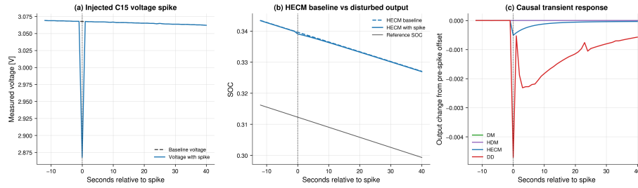
Figure 17: Causal single-cell voltage-spike response for C15 at mid-life. (a) Measured voltage with and without the injected spike, aligned to the true injection sample. (b) HECM output with its paired baseline and reference SOC. (c) Model-output change relative to the pre-spike paired offset.
