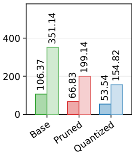
(c) Firmware flash [KiB]
