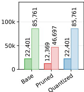
(c) Firmware flash [KiB]
