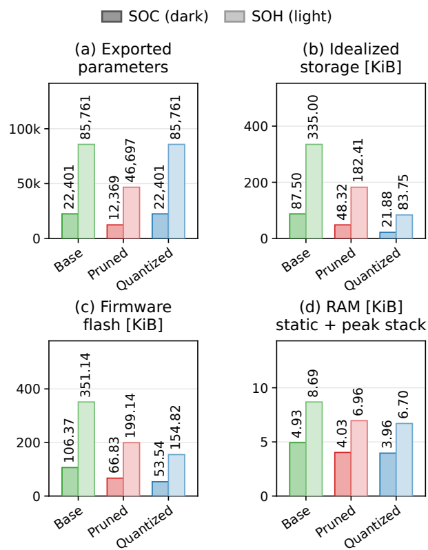
Fig. 14. Resource landscape for SOC and SOH models. The panels compare exported parameter count, idealized parameter storage, flash occupancy of the available firmware builds, and recorded static-plus-peak-stack RAM. Parameter counts include weights and merged biases in the C exports. The storage estimate assumes four bytes per parameter for Base and Pruned and one byte for Quantized. The all-INT8 estimate is idealized because the implemented quantized model retains FP32 parameters and additionally stores row scales. Dark bars denote SOC, light bars denote SOH. Memory is expressed in KiB.
