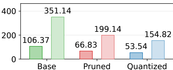
(c) Firmware flash [KiB]
