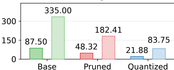
(b) Idealized storage [KiB]
