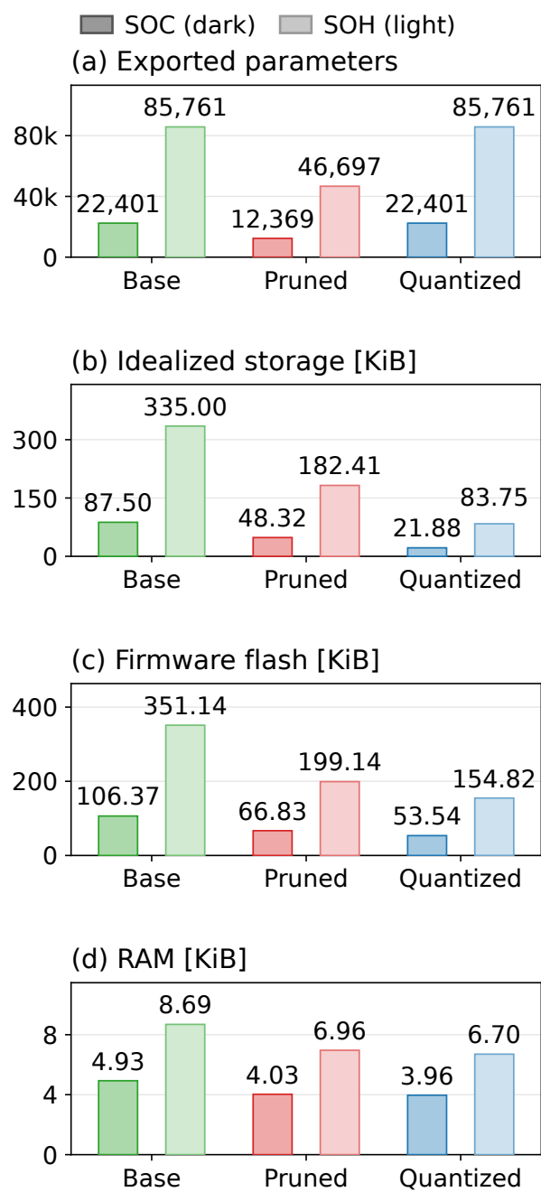
Fig. 14. Resource landscape for SOC and SOH models. The panels compare exported parameter count, idealized parameter storage, flash occupancy of the available firmware builds, and recorded static-plus-peak-stack RAM. Parameter counts include weights and merged biases in the C exports. The storage estimate assumes four bytes per parameter for Base and Pruned and one byte for Quantized. The all-INT8 estimate is idealized because the implemented quantized model retains FP32 parameters and additionally stores row scales. Dark bars denote SOC, light bars denote SOH. Memory is expressed in KiB.
