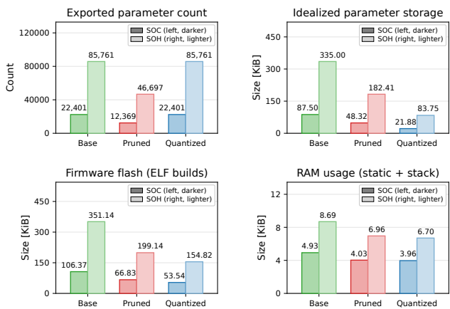
Fig. 14. Resource landscape for SOC and SOH models. The panels compare exported parameter count, idealized parameter storage, flash occupancy of the available firmware builds, and recorded static-plus-peak-stack RAM. Parameter counts include weights and merged biases in the C exports. The storage estimate assumes four bytes per parameter for Base and Pruned and one byte for Quantized. The all-INT8 estimate is idealized because the implemented quantized model retains FP32 parameters and additionally stores row scales. Dark bars denote SOC, light bars denote SOH. Memory is expressed in KiB.
