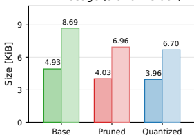
RAM usage (static + stack)
