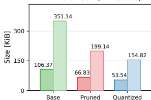
Firmware flash (ELF builds)
