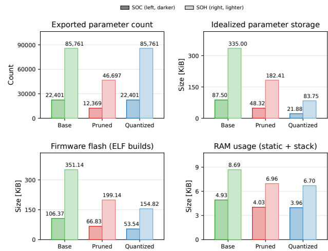
Fig. 14. Resource landscape for SOC and SOH models. The panels compare exported parameter count, idealized parameter storage, flash occupancy of the available firmware builds, and recorded static-plus-peak-stack RAM. Parameter counts include weights and merged biases in the C exports. The storage estimate assumes four bytes per parameter for Base and Pruned and one byte for Quantized. The all-INT8 estimate is idealized because the implemented quantized model retains FP32 parameters and additionally stores row scales. Dark bars denote SOC, light bars denote SOH. Memory is expressed in KiB.
