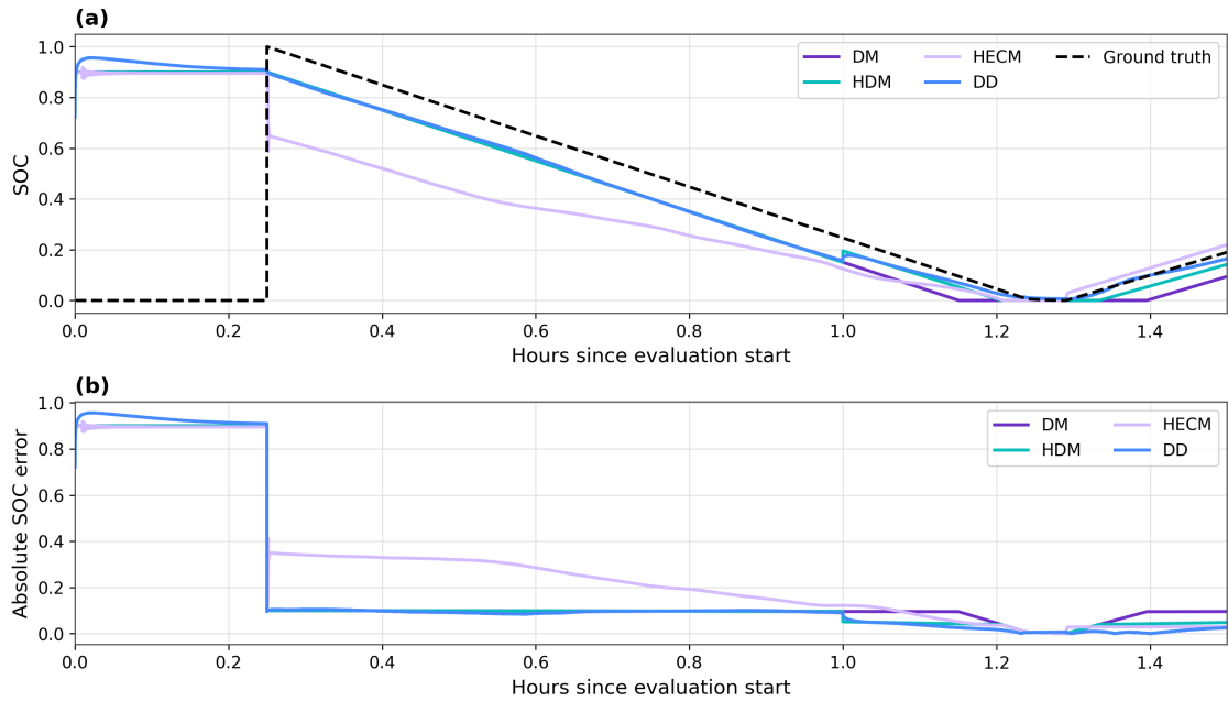
Abbildung 6.8: Recovery after initialization mismatch in a reset-free evaluation window. The figure shows the disturbed SOC trajectories after the imposed initial-state error together with the corresponding absolute SOC error over time, so that re-synchronization to the baseline-relative recovery bands becomes directly visible. This local view is required because full-run averages alone do not capture restart behavior adequately.
