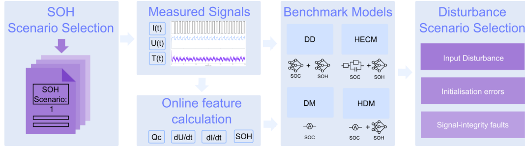
Abbildung 6.2: Methodology overview of the robustness benchmark. Measured current, voltage, temperature, and time signals are first converted into causal online auxiliary quantities such as cumulative charge Q_c , derivative channels, equivalent full cycles EFC, and shared SOH context. The resulting online stream is then processed by the four estimator classes under matched execution conditions, exposed to measurement-only disturbance scenarios, and finally evaluated through global and local performance metrics that separate baseline accuracy, convergence behavior, and disturbed-operation robustness.
