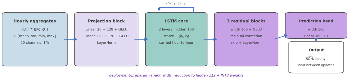
Abbildung 6.3: Block-level architectures of the data-driven estimator components used in the benchmark. (a) The DD SOC estimator processes the eight online input channels with a single stateful GRU layer of hidden size 96, followed by an MLP head with one ReLU-activated hidden layer of size 96 and a sigmoid output. (b) The shared SOH estimator forms a 20-dimensional hourly feature vector by computing four statistics for each of the five causal base signals \{U, I, T, \text{EFC}, Q_c\} , projects this vector through a two-layer feature-projection block of width 128, processes the projected sequence with a two-layer stateful LSTM of hidden size 160, and maps the recurrent representation through three residual MLP blocks and a prediction head of width 160. The deployment-prepared variants used in the benchmark are described in Section 6.5.4.
