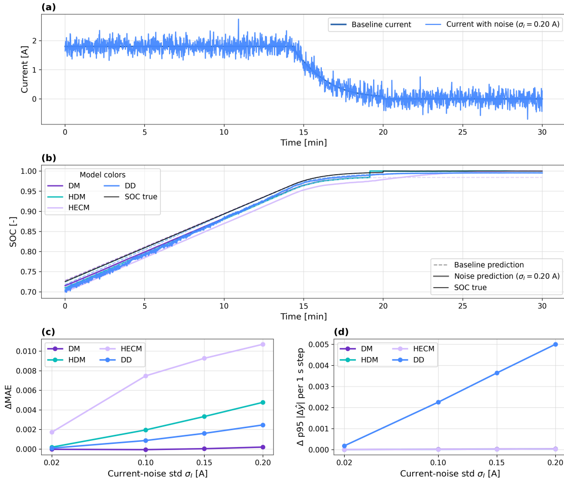
Abbildung 6.7: Noise sensitivity under additive current noise. The figure combines a representative disturbed window, a matched SOC comparison in the same interval, the global MAE penalty in the compact benchmark matrix, and the local output-variability trend across an extended current-noise sweep. This makes visible that zero-mean current noise is mainly a local disturbance-propagation test rather than the same type of long-term drift test as persistent current bias.
