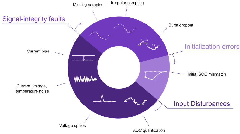
Abbildung 6.4: Disturbance taxonomy used in the robustness benchmark. Input disturbances, initialization mismatch, and measurement-continuity faults are separated so that drift, loss of correction, delayed recovery, and transient instability can be interpreted as different estimator-side effects.
