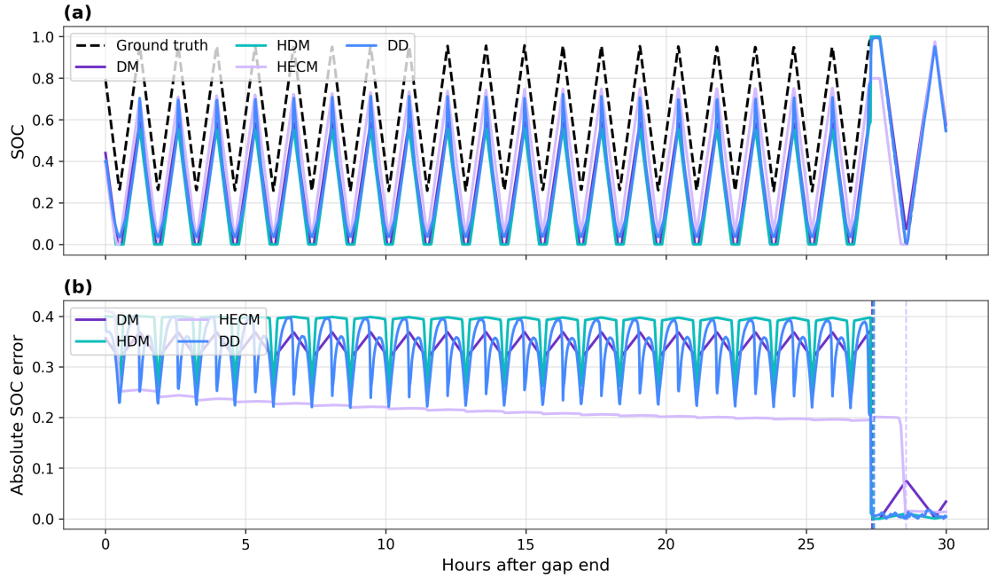
Abbildung 6.11: Post-gap recovery after burst dropout. The figure shows the disturbed SOC trajectories after the frozen interval together with the corresponding absolute SOC error, so that the delayed return toward the baseline bands becomes directly visible. It therefore complements the moderate full-run \Delta\text{MAE} values with the practically more revealing local recovery behavior.
