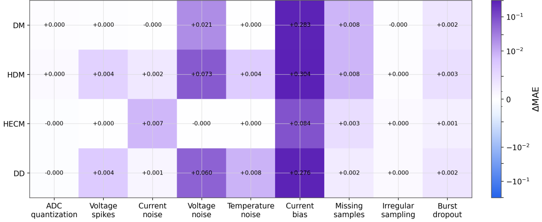
Abbildung 6.13: Cross-scenario error increase relative to the baseline case. The heatmap condenses the disturbed-scenario penalties, including the ADC-quantization case, and makes estimator-specific ranking shifts visible across disturbance classes. It therefore serves as the compact scenario-overview view for identifying where robustness advantages are stable and where they are disturbance-specific. Error values in the figure are SOC fractions on a 0 to 1 scale. Multiplication by 100 gives percentage points.
