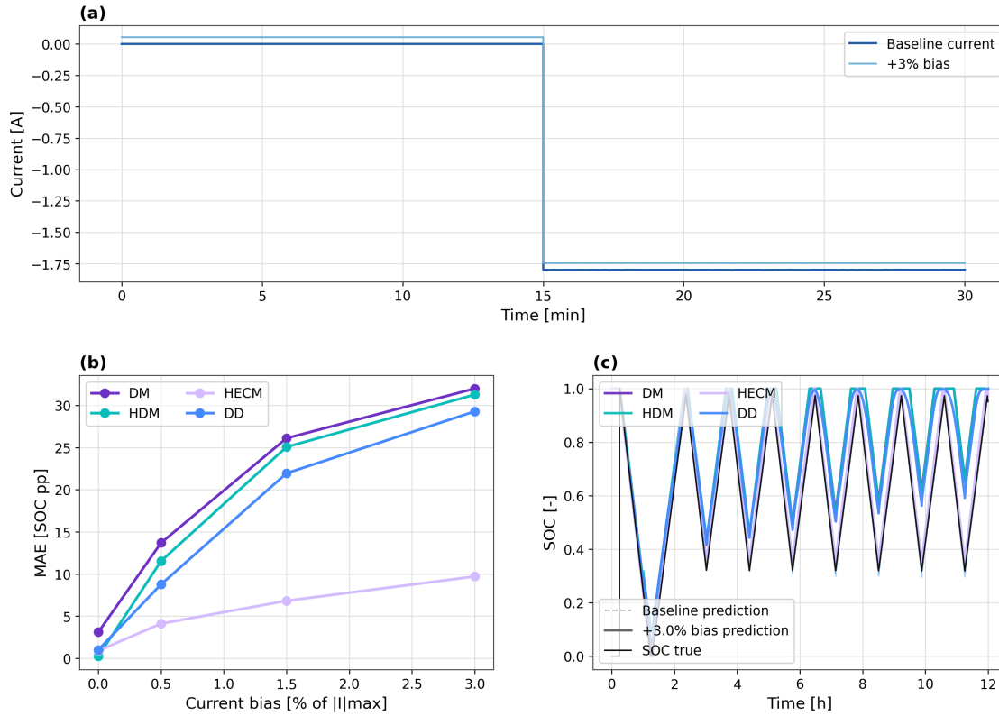
Abbildung 6.6: Sensitivity to current-measurement bias. The figure combines a representative local example of the applied bias, the global degradation of SOC accuracy across the matched bias sweep, and the resulting SOC divergence over time for a strongly biased case. Together, these views show why persistent current bias clearly separates the integration-based estimators from the voltage-corrected observer variant.
