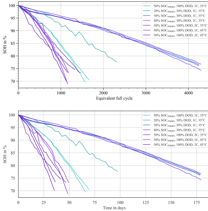
Abbildung 5.1: SOH progression of the 14 cells over equivalent full cycles and over absolute time.
