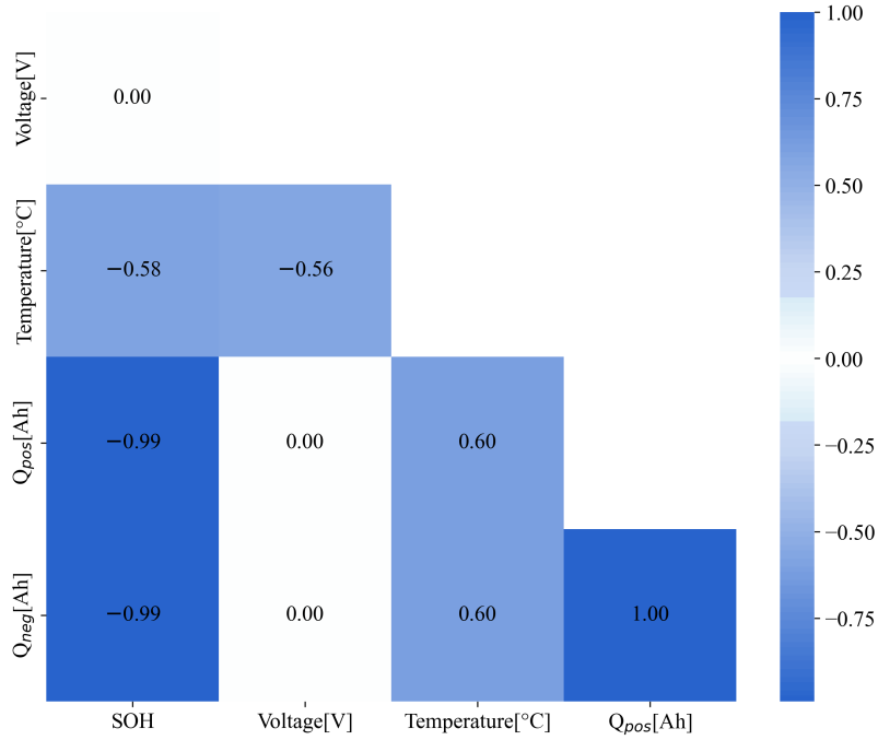
Abbildung 5.2: Correlation heatmap used to identify direct linear relations between SOH and candidate input variables.
