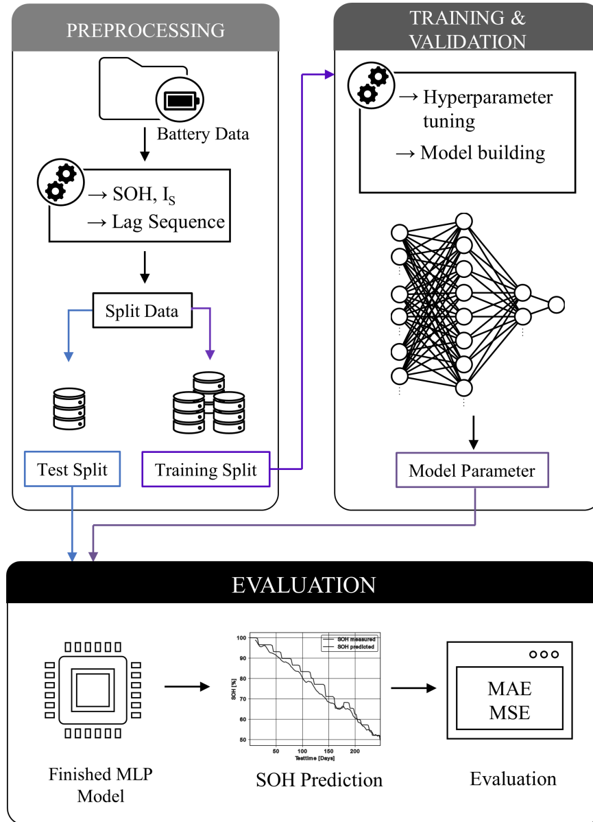
Abbildung 5.4: Processing and evaluation workflow of the MLP-based SOH estimator.
