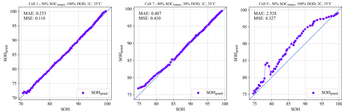
Abbildung 5.8: Predicted versus measured SOH values for the representative test cells.
