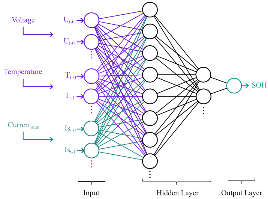
Abbildung 5.5: MLP architecture used for SOH estimation.
