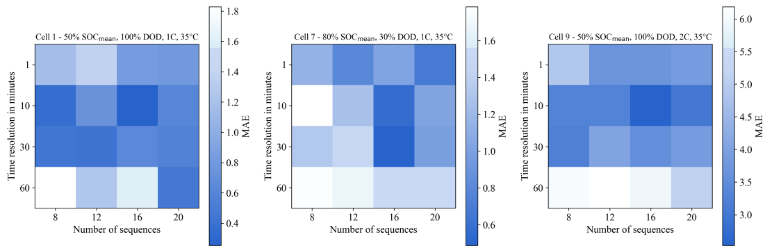
Abbildung 5.6: MAE matrix showing the interaction between sequence length and temporal resolution.
