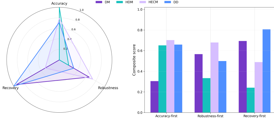
Figure 13: Decision-oriented synthesis of the benchmark results. Panel (a) collapses the benchmark into three normalized decision dimensions, namely nominal accuracy, disturbed-scenario robustness, and recovery behavior. Panel (b) shows three illustrative deployment-priority profiles and is intended only as a visual complement to Table 4, not as a replacement for the raw scenario metrics.
