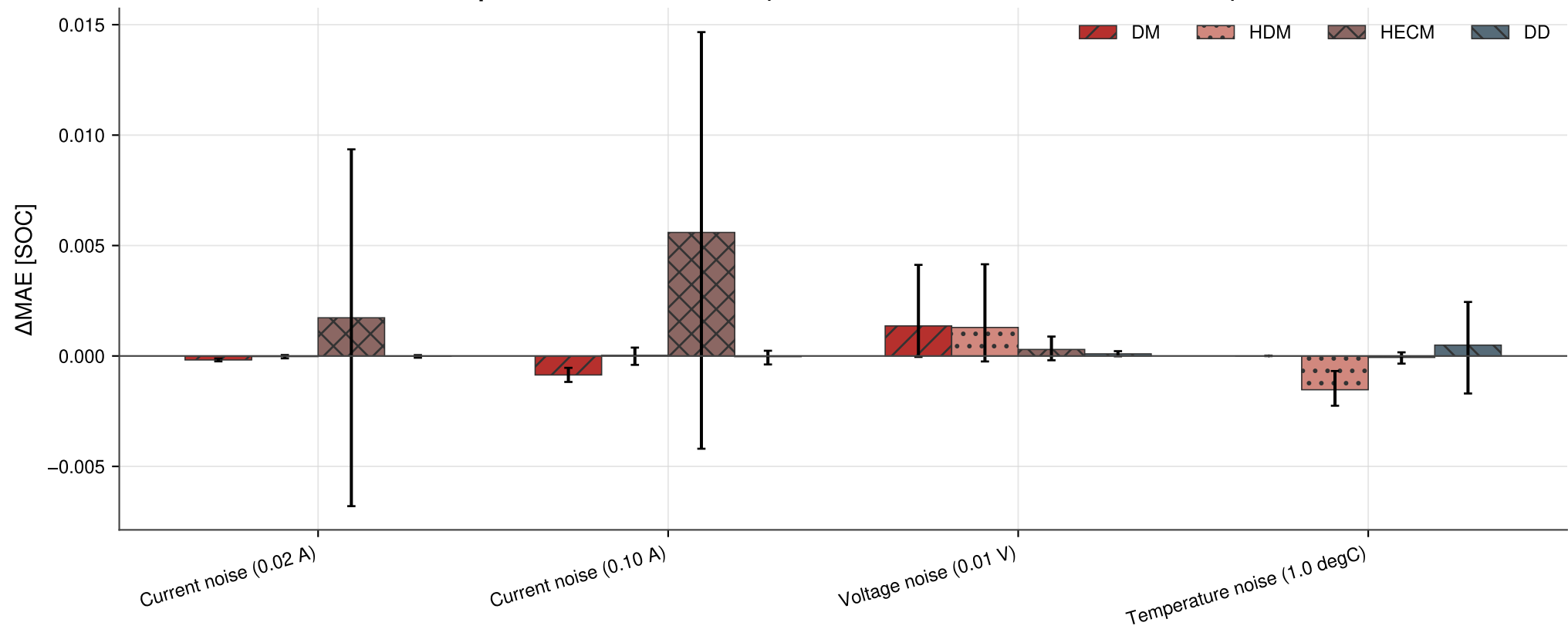
Repeated noise robustness (cell-macro mean and hierarchical 95% CI)
