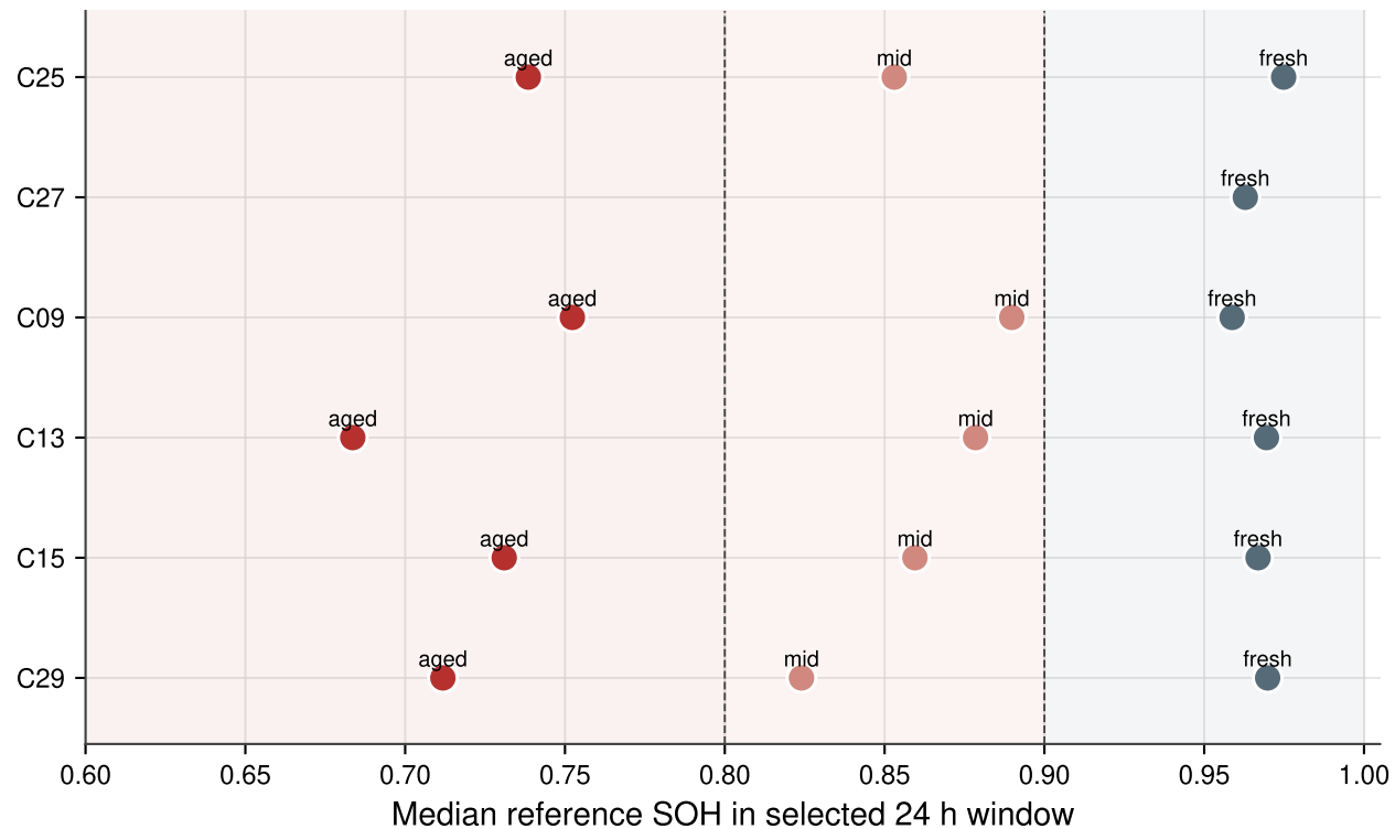
16 frozen cell/SOH evaluation windows
