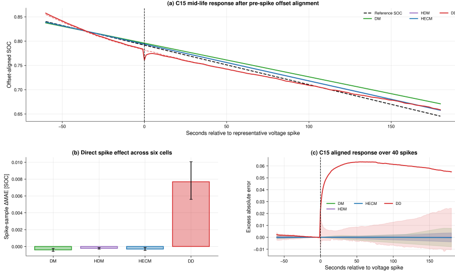
Figure 17: Voltage-spike response using current C15 and six-cell evidence. (a) Representative C15 mid-life trajectories aligned to the true injection sample and corrected only for each model’s constant mean pre-spike baseline offset; dashed model lines are paired baselines and solid lines are disturbed outputs. (b) Mean spike-sample \Delta MAE across six cells with 95% bootstrap confidence intervals. (c) Mean C15 excess absolute error aligned over 40 spikes; shaded bands show the interquartile range.
