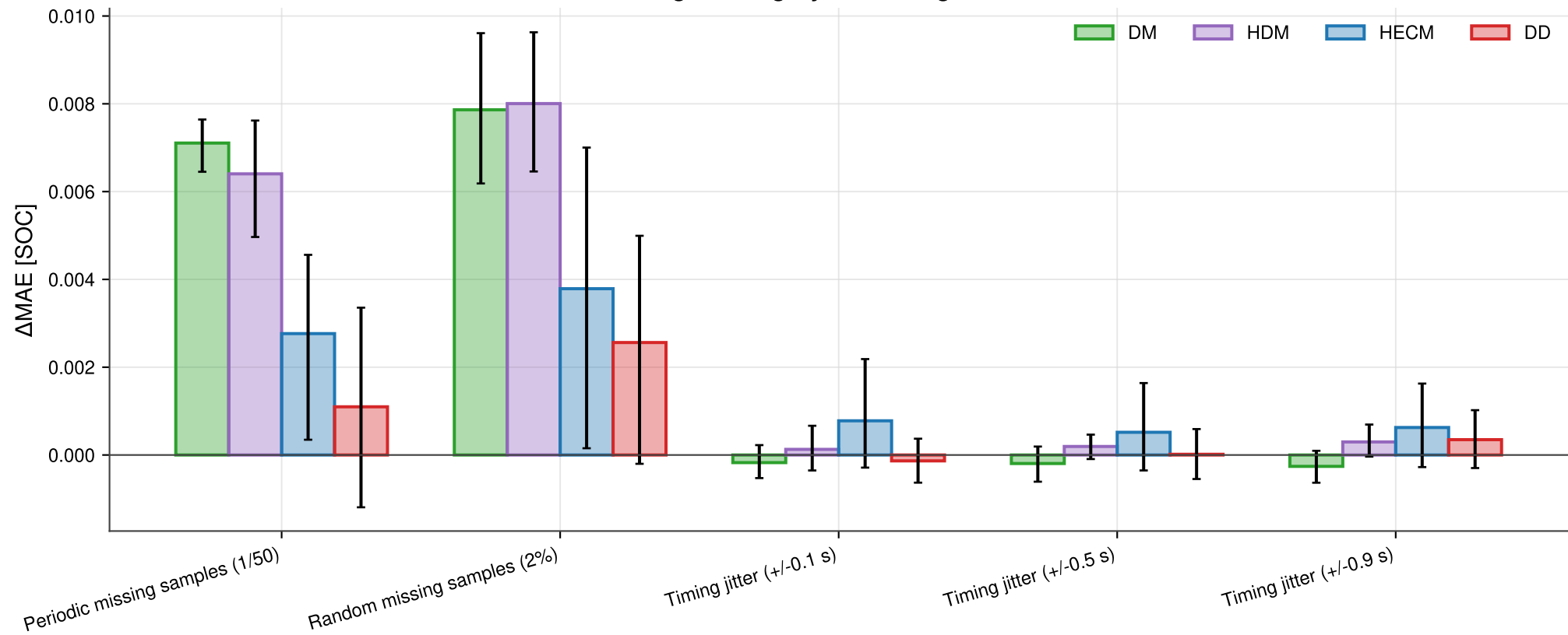
Signal-integrity and timing stress
