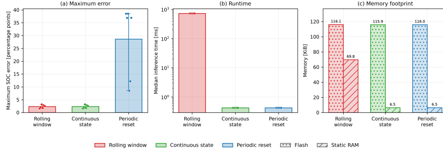
Figure 20: DD inference-mode trade-off on the STM32. The panels compare maximum dataset-SOC error, median latency, and linker-reported firmware memory for exact rolling-window, continuous-state, and periodically reset recurrent execution. Cell points show that periodic resets, not continuous forwarding, create the dominant accuracy loss.
