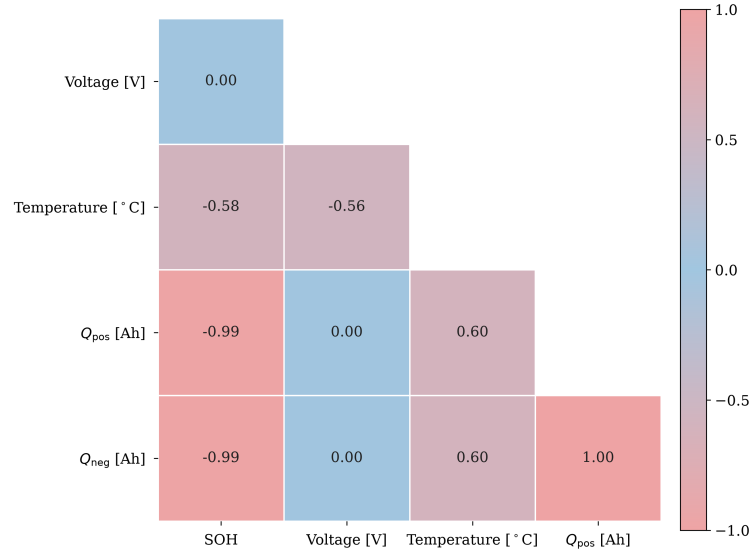
Figure 4.1: Correlation heatmap illustrating the linear relation between SOH and candidate input variables, including temperature and cumulative current Q in positive and negative direction. The symmetric OKLAB scale maps zero correlation to blue and increasing absolute correlation magnitude toward red. Consequently, coefficients of -1 and +1 receive the same red endpoint colour, while the sign and exact value remain visible in the printed coefficient.
