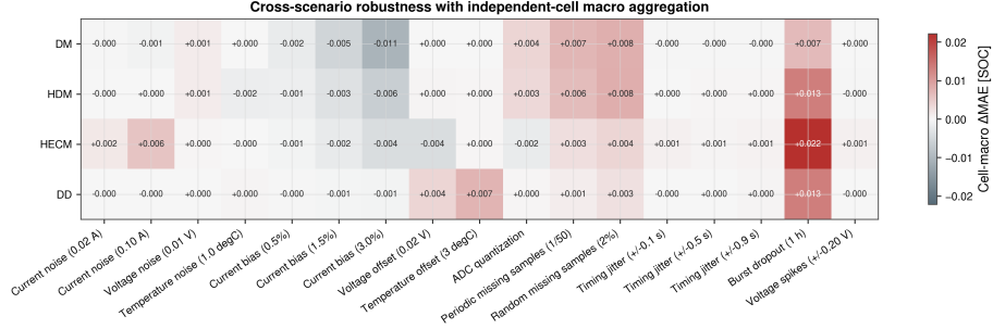
Figure 18: Cross-scenario error increase relative to the baseline case. The heatmap summarizes the disturbed-scenario \Delta MAE values, including ADC quantization, and highlights where robustness rankings change across disturbance classes.
