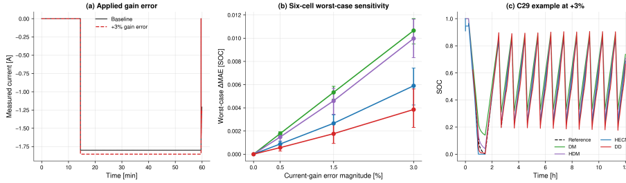
Figure 12: Current-gain sensitivity. (a) Representative measured-current segment before and after the +3% gain error. (b) Six-cell worst-case MAE change, retaining the adverse direction from each matched \pm b pair; error bars show 95% bootstrap confidence intervals across cells. (c) Representative C29 mid-life SOC trajectories at +3%.
