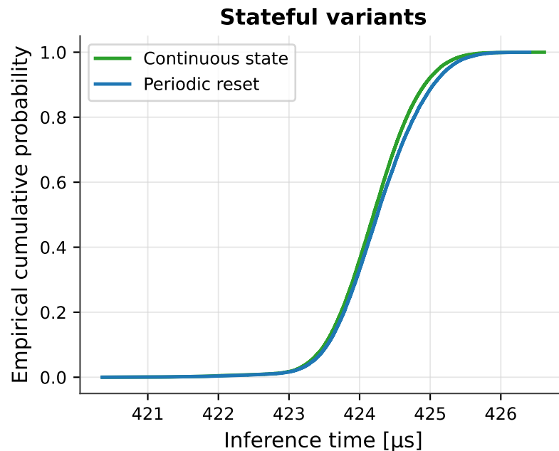
Measured STM32 inference-time distributions and C27 repeatability
