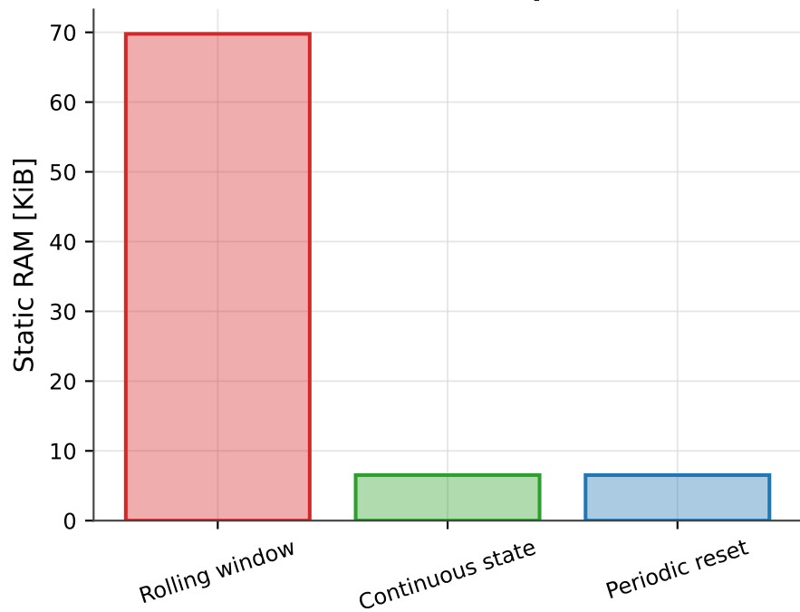
Static RAM footprint
