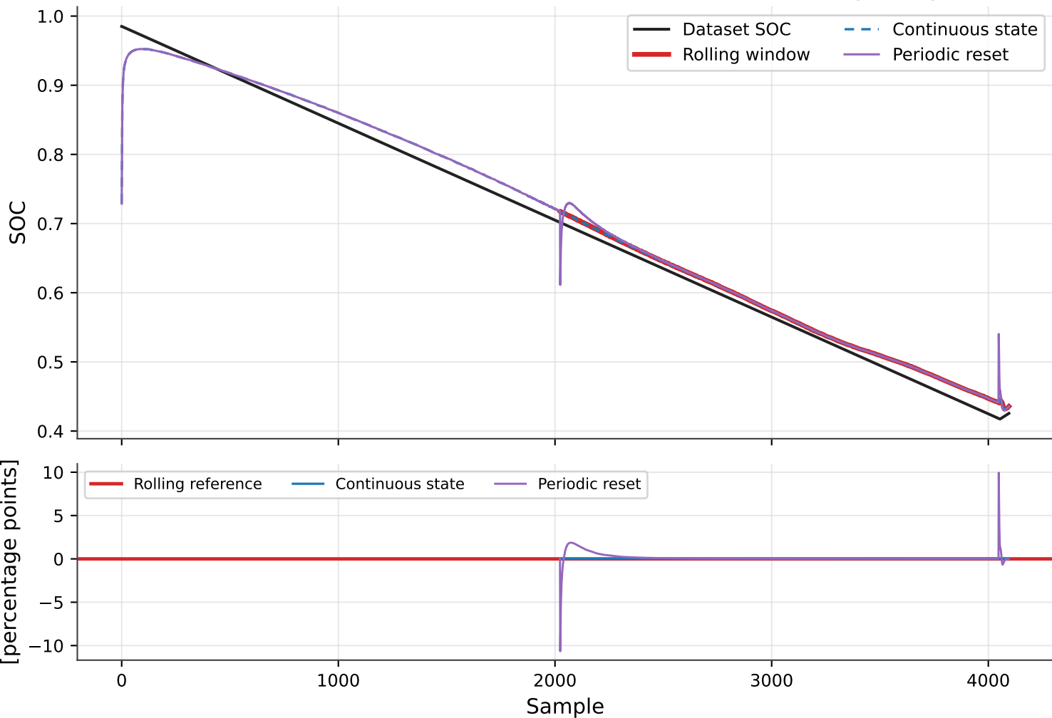
DD inference modes over the complete benchmark trajectory
